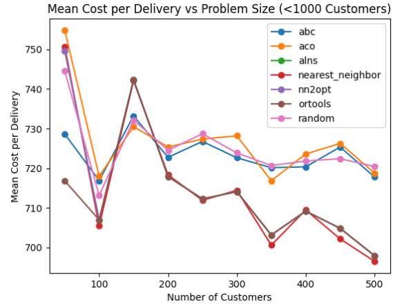
Fig. 2. Mean cost per delivery across solvers for small-scale instances ( n < 1000 customers).
