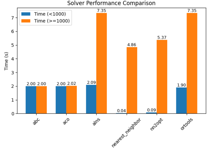
Fig. 4. Analysis of Solver Execution Times: Comparing Small-Scale ( n < 1000 ) vs. Large-Scale ( n \geq 1000 ) Performance.
